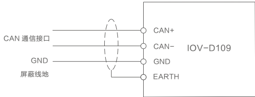
CANopen通讯适配卡配线图
